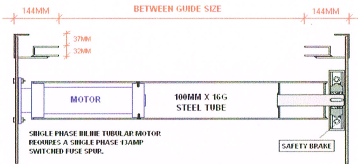
PLAN VIEW OF BARREL, MOTOR AND SAFETY BRAKE
